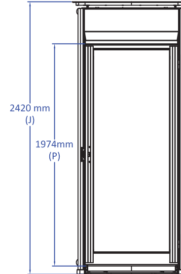
Trio+ Lift with Shaft lid (Full Height Door)
