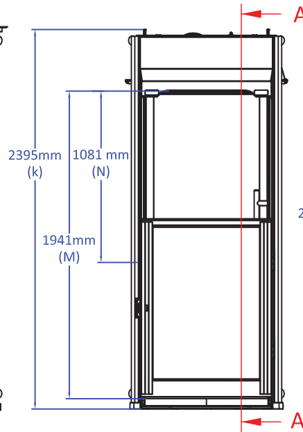
Trio+ Lift without Shaft lid (Half Height Door)
