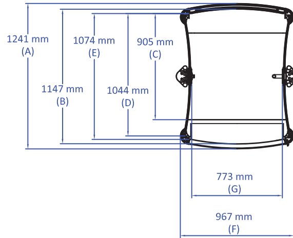
Trio+ Lift Top View
