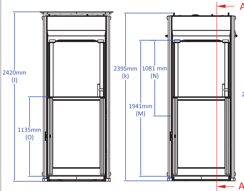
Trio+ Lift with Shaft lid (Half Height Door)
