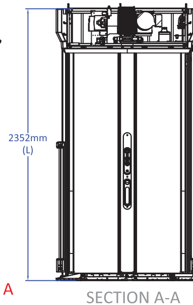
Trio+ Lift without Shaft lid (Half Height Door)
