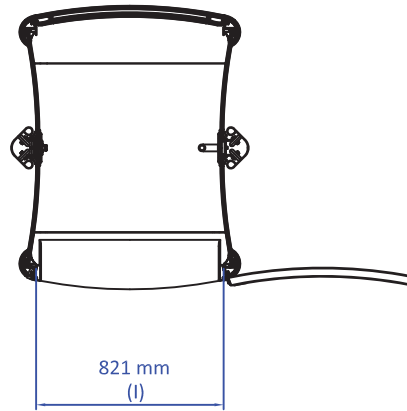
Trio+ Lift Top View 180° Door Opening
