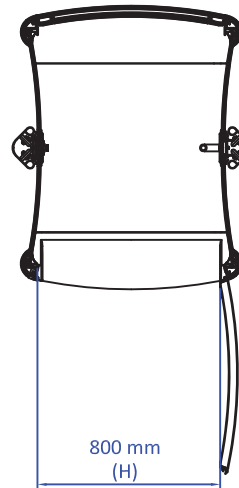
Trio+ Lift Top View 90° Door Opening
