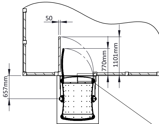
SECTION K-K
